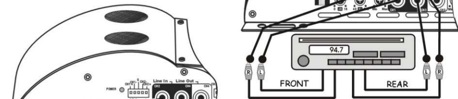
FOUR CHANNEL SIGNAL CONNECTIONS (RADIO WITH FRONT AND REAR OUTPUTS)
